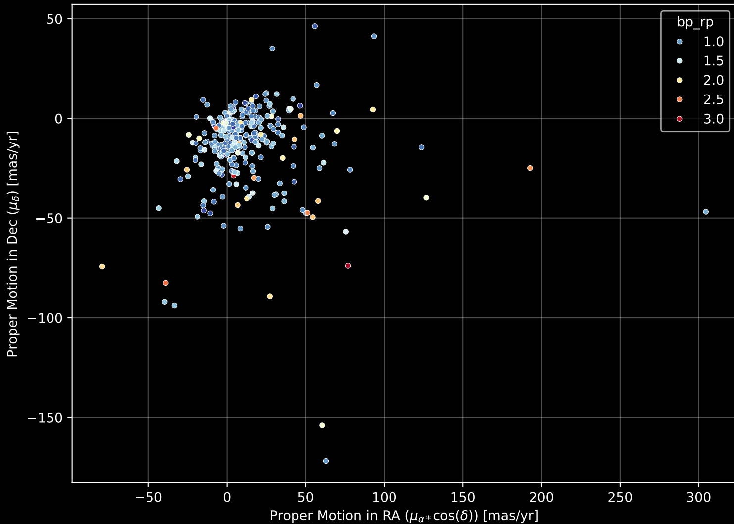
APOGEE DR17 Field: [137-71] Proper Motion Diagram (n= 292)
