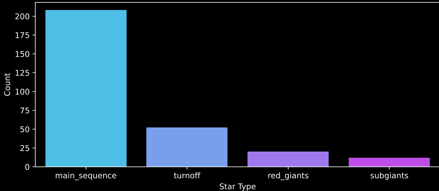
APOGEE DR17 Field: [137-71] Count plot of Star Type
