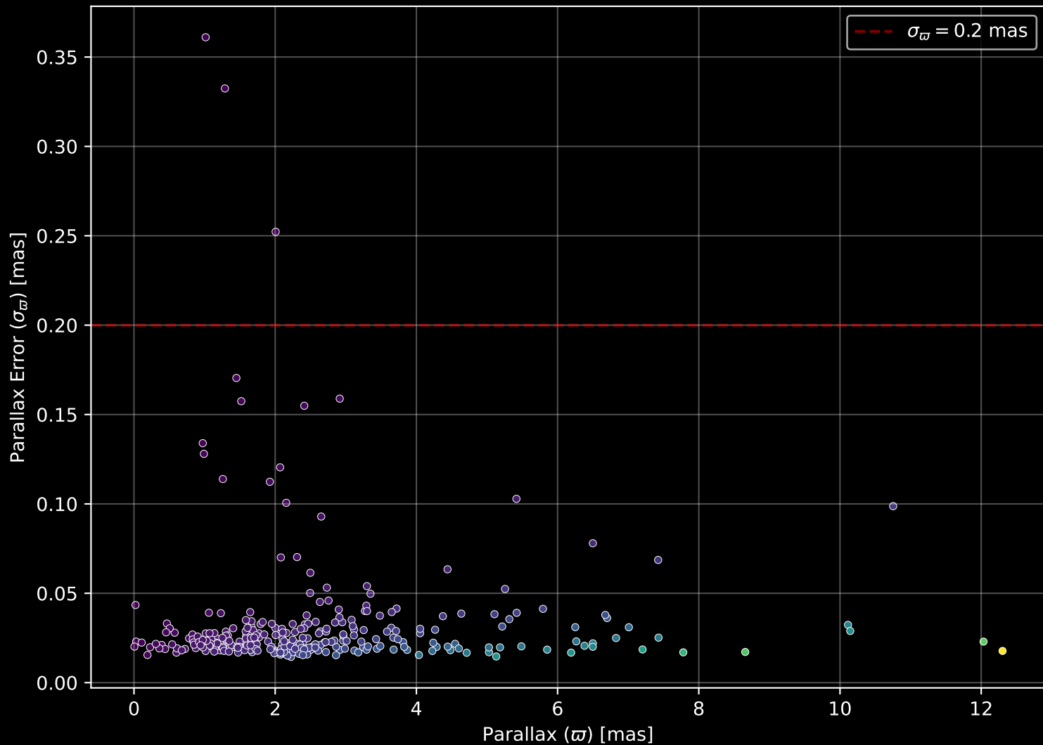
APOGEE DR17 Field: [137-71] Parallax Quality (n= 292)
