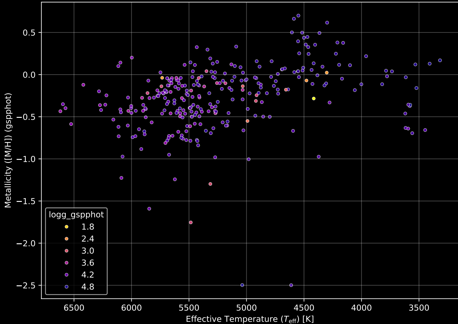
APOGEE DR17 Field: [137-71] Stellar Population Parameters (n= 292)
