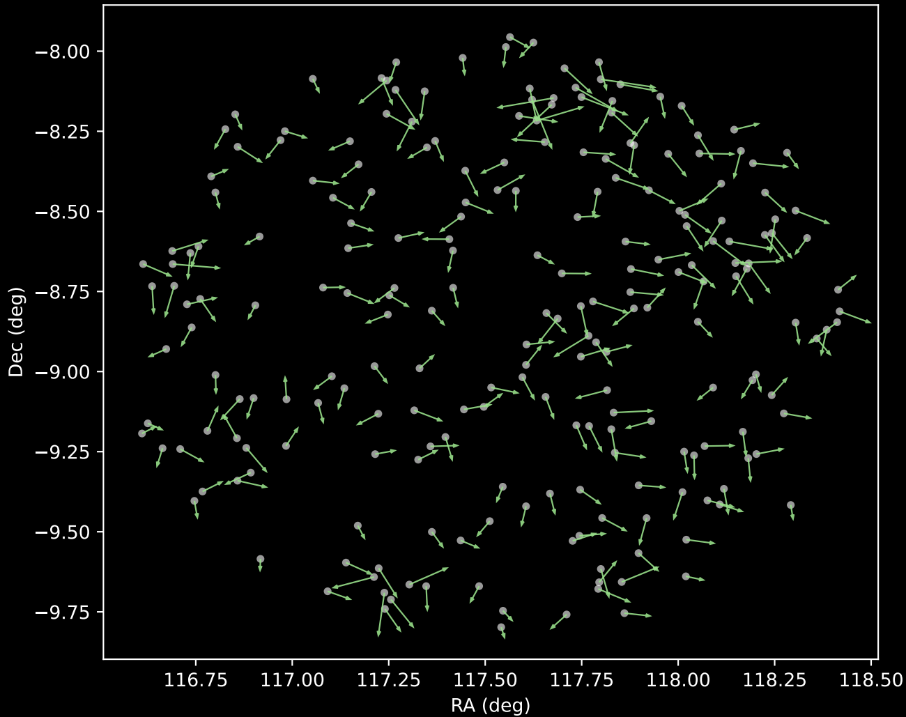
APOGEE DR17 Cluster 5 Proper Motion Vectors (n=224)
