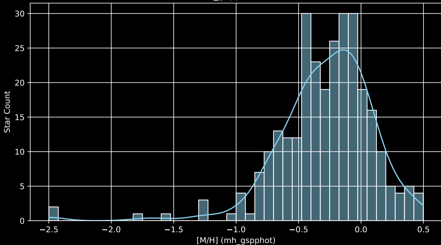
APOGEE DR17 Field: [137-71 [M/H] (mh_gspphot) (n= 288)
