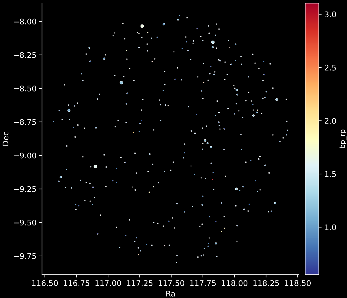
APOGEE DR17 Field: [137-71] Stars: 292
