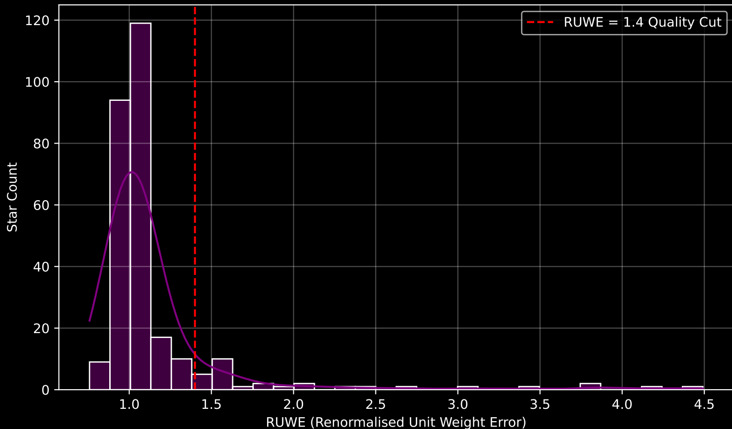
GAPOGEE DR17 Field [137-71] RUWE Distribution (n= 279)
